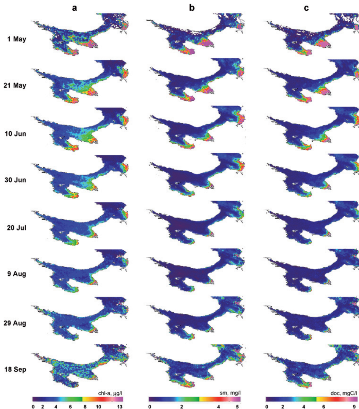
Figure 6: Based on a regionally tuned algorithm the spatiotemporal variability of satellite-retrieved concentrations of: (a) chlorophyll chl ; (b) suspended minerals sm ; and (c) dissolved organic content doc , are made for the White Sea in northwest Russia. The data are merged into 20 day periods throughout the phytoplankton vegetation season from May-September during the years 1997 to 2004. The time-series reveals a significant trend in the ecosystem parameters of the White Sea during the 7 years investigation period. From: Pozdnyakov, D. V., O. M. Johannessen, A. A. Korosov, L. H. Pettersson, H. Grassl, and M. W. Miles (2007), Satellite evidence of ecosystem changes in the White Sea: A semi-enclosed arctic marginal shelf sea, Geophys. Res. Lett. , 34, L08604, doi:10.1029/2006GL028947. 2007 © American Geophysical Union – Reproduced by permission of American Geophysical Union
