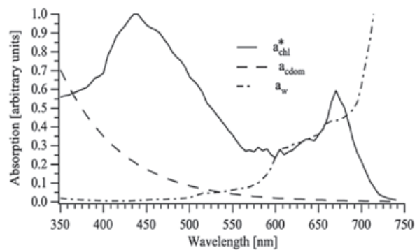
Figure A1. Qualitative comparisons between the absorption spectrum of pure water, a_w(\lambda) , a chlorophyll specific absorption spectrum of phytoplankton pigment concentration, a^*_{chl}(\lambda) (Prieur and Sathyendranath, 1981), and a typically exponential absorption spectrum of CDOM, a_{cdom}(\lambda) (Bricaud et al. 1981).
